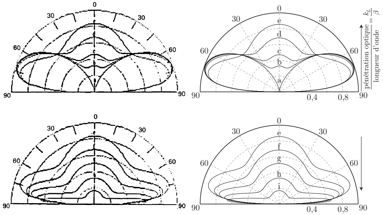
Figure 9 Variation of the longitudinal directivity pattern with k_L/b for k_1 \ll 1 and Poisson's ratio \sigma = 0.23 . k_1/b are, respectively, (a) 0.01; (b) 0.2; (c) 0.3; (d) 0.5; (e) 1; (f) 2; (g) 3; (h) 5; (i) 10
